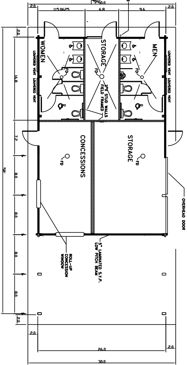
FLOOR/ROOF PLAN SCALE: 1/4"=1'-0"
